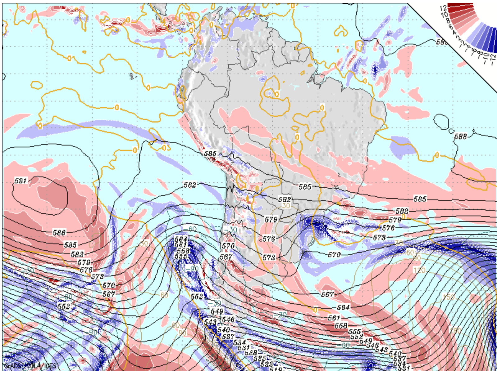
120Hr GFS Issued: 00Z19AUG2011 Valid: 00Z Wed 24 AUG 2011 500mb Heights (dam), Vorticity ( 10^{-5}/\text{sec} ), 12hr Hgt Change (m)
