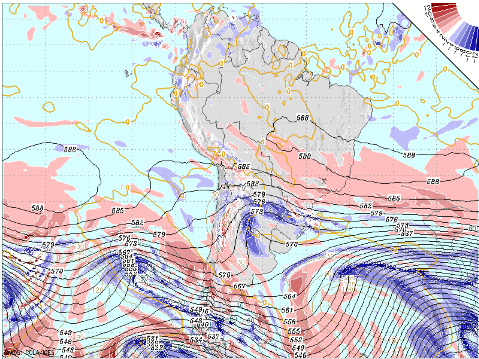
96Hr GFS Issued: 00Z19AUG2011 Valid: 00Z Tue 23 AUG 2011 500mb Heights (dam), Vorticity ( 1e^{-5}/\text{sec} ), 12hr Hgt Change (m)
