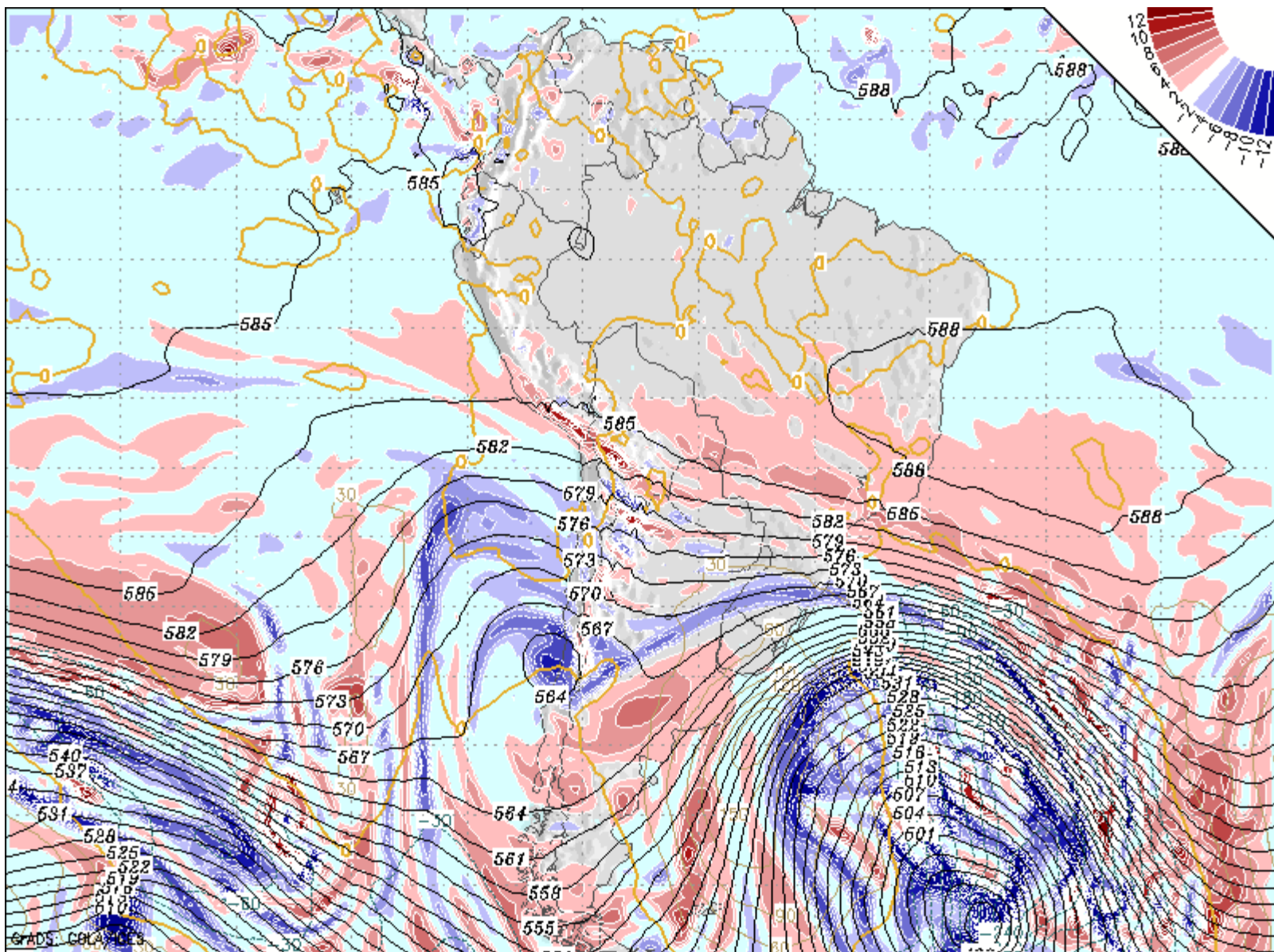
48Hr GFS Issued: 00Z19AUG2011 Valid: 00Z Sun 21 AUG 2011 500mb Heights (dam), Vorticity ( 1e^{-5}/\text{sec} ), 12hr Hgt Change (m)
